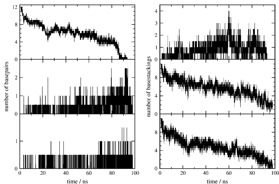
FIGURE 4 (Left) Average number of WC interstrand basepairs as a function of time (top) from the two trajectories. Number of intrastrand basepairs on the A-strand (middle) and T-strand (bottom). (Right) Average number of interstrand base stackings as a function of time (top) from the two trajectories. Number of intrastrand base stackings on the A-strand (middle) and T-strand (bottom).
